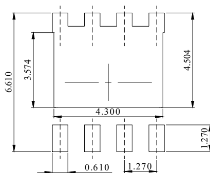
DIMENSIONS: MILLIMETERS
