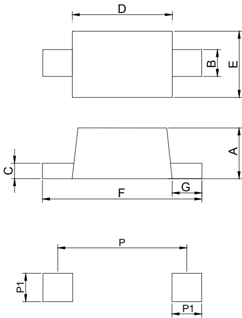
Land Pattern
